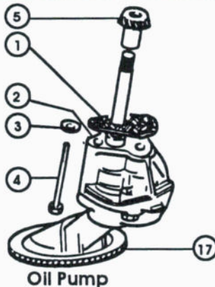
Oil Pump
