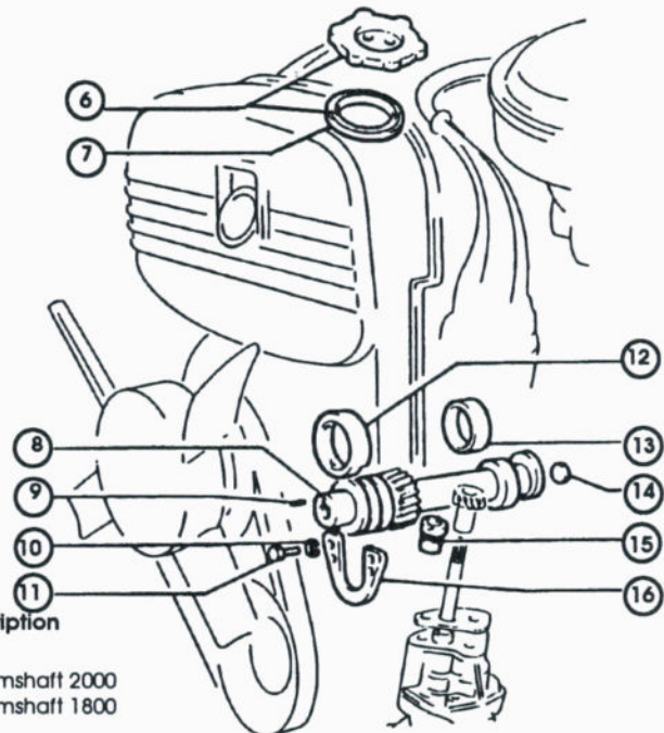
Auxiliary Camshaft
