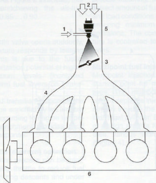
Fig. 5: Single-point fuel injection (TBI)
