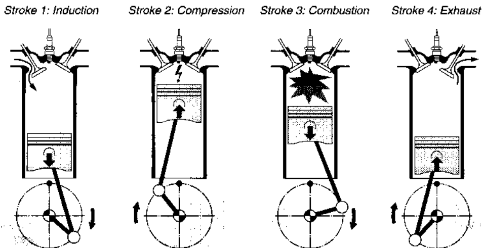
Fig. 2: Operating cycle of the four-stroke spark-ignition engine
