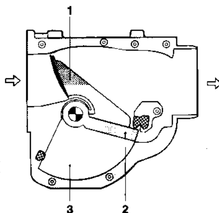
Fig. 33: Air-flow sensor of the L3-Jetronic 1 Sensor flap, 2 Compensation flap, 3 Damping volume.
